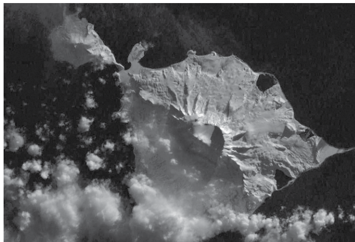
Aerial view of Heard Island, with Big Ben at its centre.
