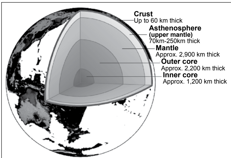
Structure of the Earth
