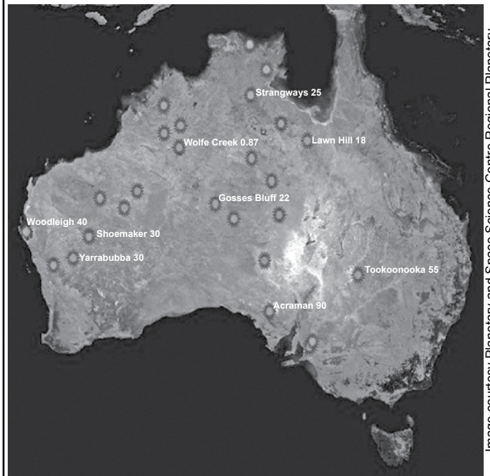
A map of known Australian impact craters with some labelled with their diameters (in kilometres)
